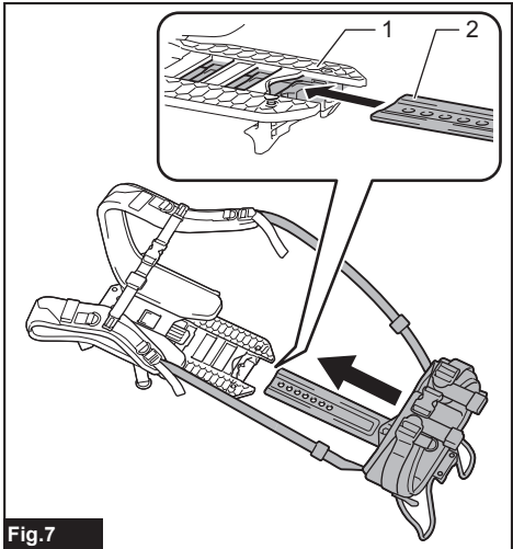
► 1. Plate of shoulder harness 2. Base plate
